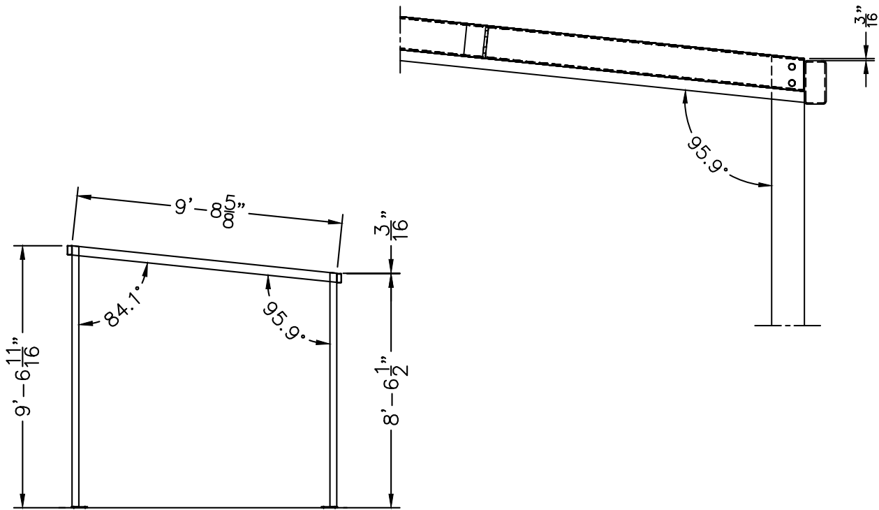
SECTION VIEW
