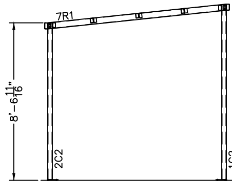
RIGHT END ELEVATION VIEW FROM INSIDE
